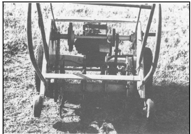
Figure 12. A power aerator.
